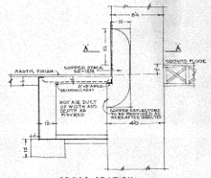
CROSS SECTION
