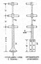
DETAILS OF GALLERY BRACKETS, ETC.
