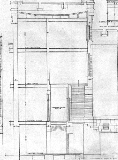
SECTION THRO' ENTRANCE
