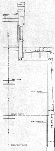
SECTION
