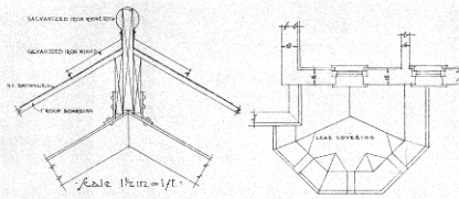
DETAIL OF RIDGE OF MAIN HALL ROOF
