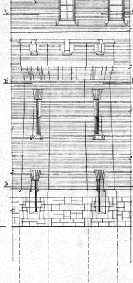
ELEVATION OF OCTAGONAL EXTENSION
