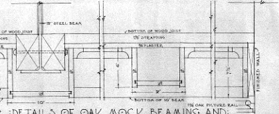
DETAILS OF OAK MOCK BEAMING AND CORNICE IN COMBINED OFFICERS ANTE AND ASSEMBLY ROOMS
