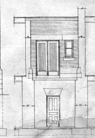
SECTION THRO' RECESS TO ENTRANCE
