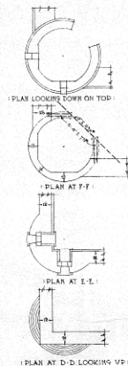
PLAN AT D-D LOOKING UP
