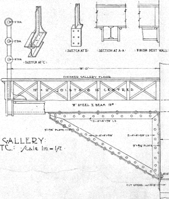
LONGITUDINAL SECTION DETAILS OF BOWLING ALLEY BEDS
